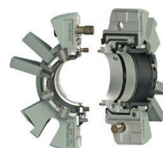
Mechanical Seals
